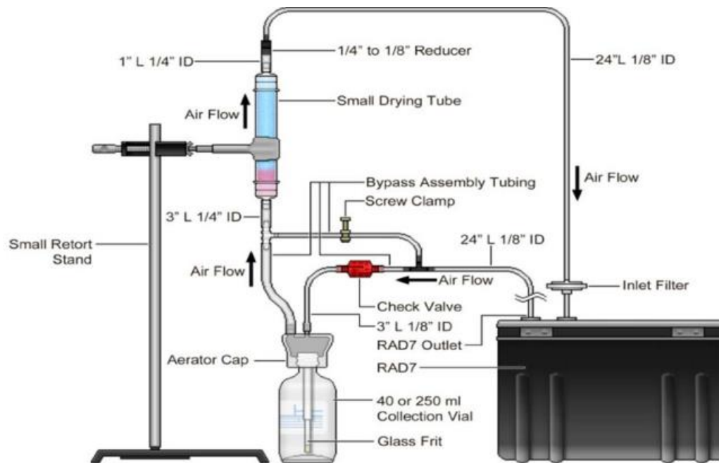
Fig.4. RAD-7 experimental setup to measure the concentration of radon activity [38]
