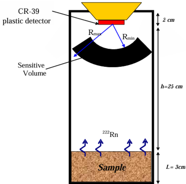
Fig.3. Experimental setup for the measuring of radon exhalation [34]
