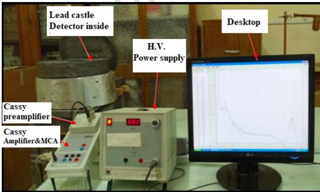
Fig.2. The components of NaI (Tl) gamma-ray spectrometry system
