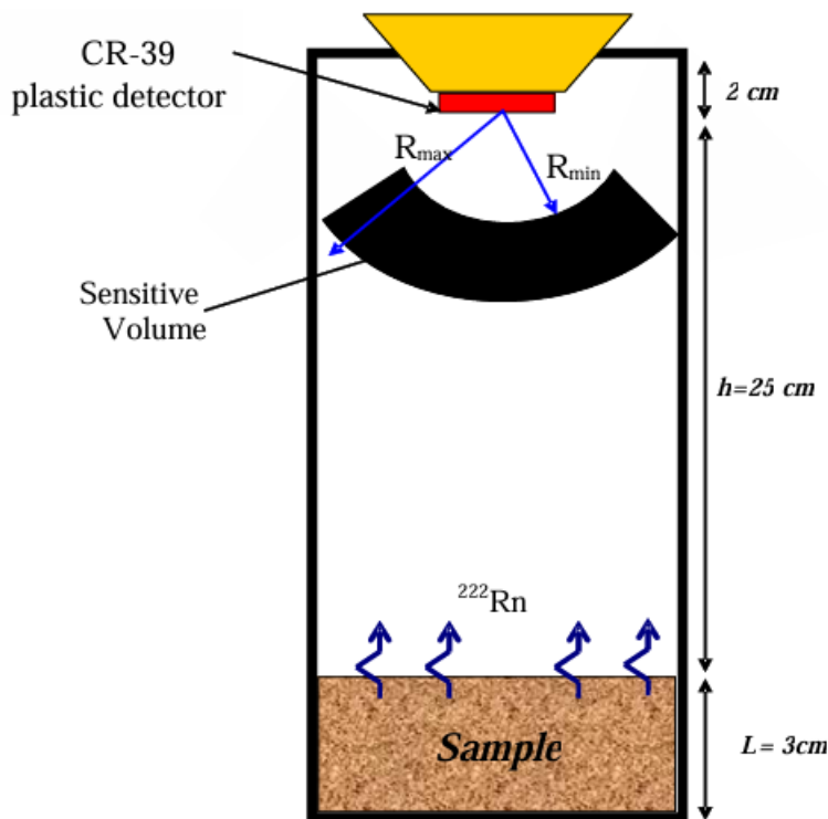
Fig.3. Experimental setup for the measuring of radon exhalation [25]
