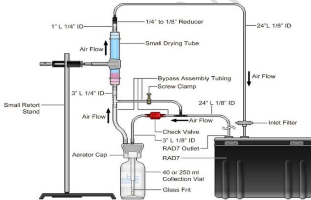
Fig.4. RAD-7 experimental setup to measure the concentration of radon activity [29]
