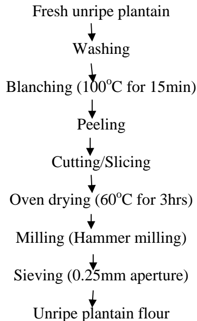
Figure .3: Flowchart for the production of unripe plantain flour
