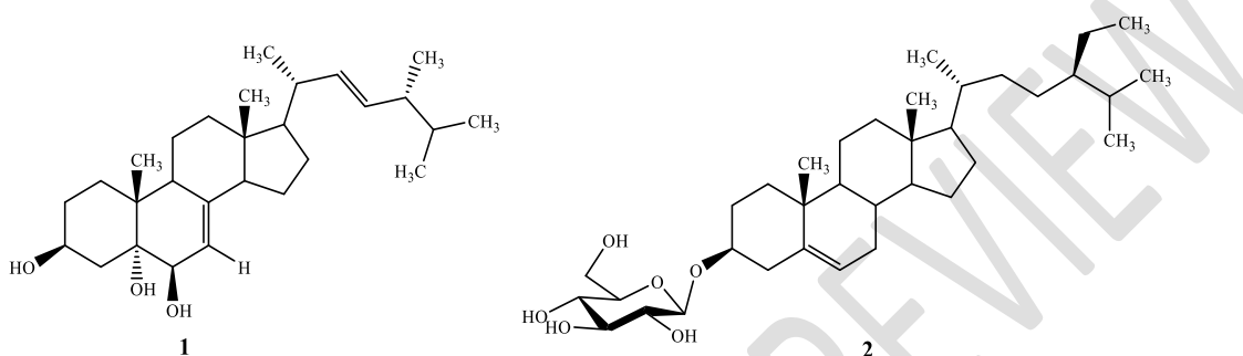
Figure 1: Chemical structures of compounds 1 and 2 . (1): cerevisterol; (2): \beta -sitosterol -3-O- \beta -D-glucopyranoside.
