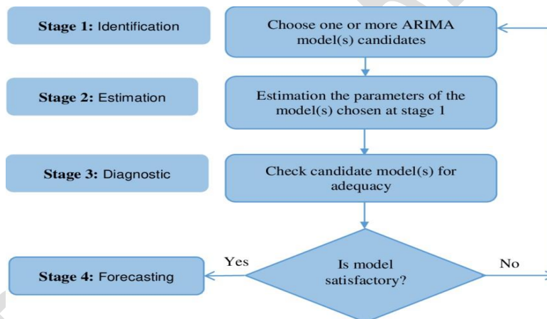
Fig.2. Flow chart of Box-Jenkins Methodology
