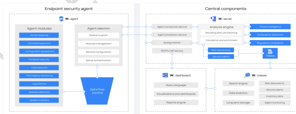
Fig. 4: Wazuh architecture [13].
