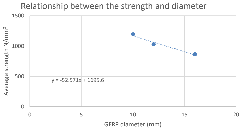
Figure 3a: Relationship between tensile strength and diameter of GFRP bar (Rupture failure)
