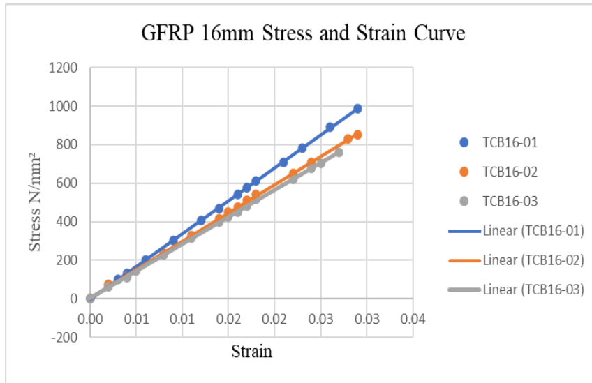
Figure 8a: Stress and strain curve for 16mm GFRP bar (rupture failure)
