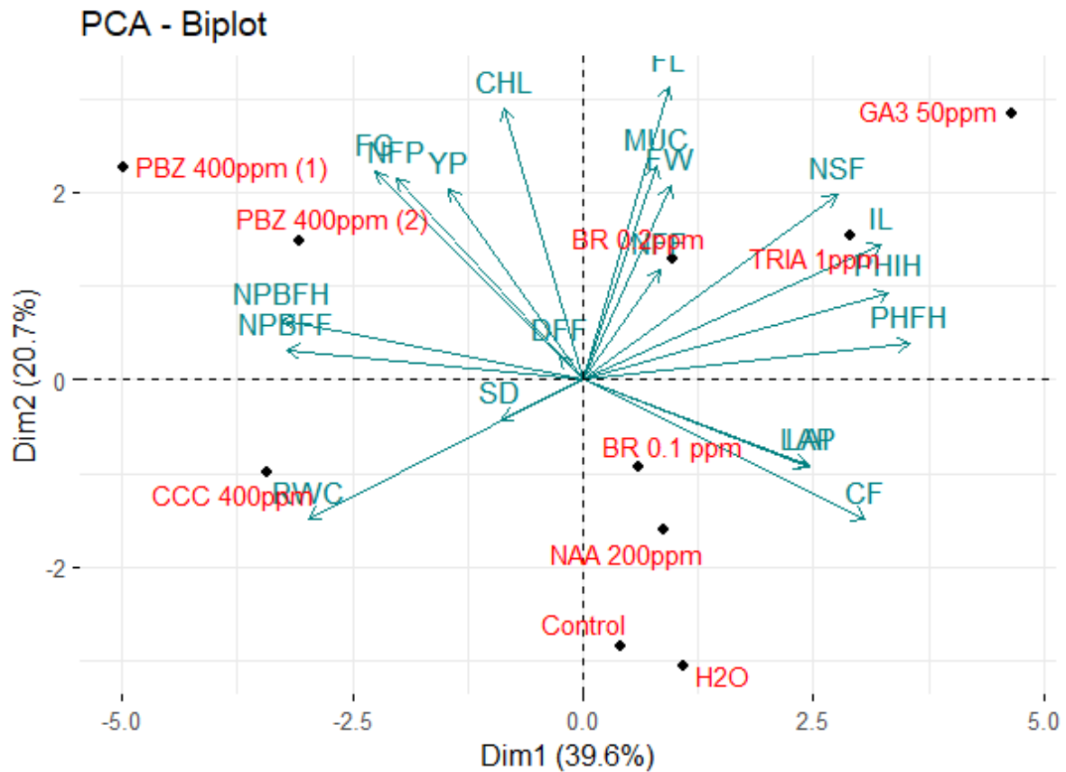
Fig. 3. Treatment-by-traits biplot showing plant growth regulators – plant traits interactions in okra
