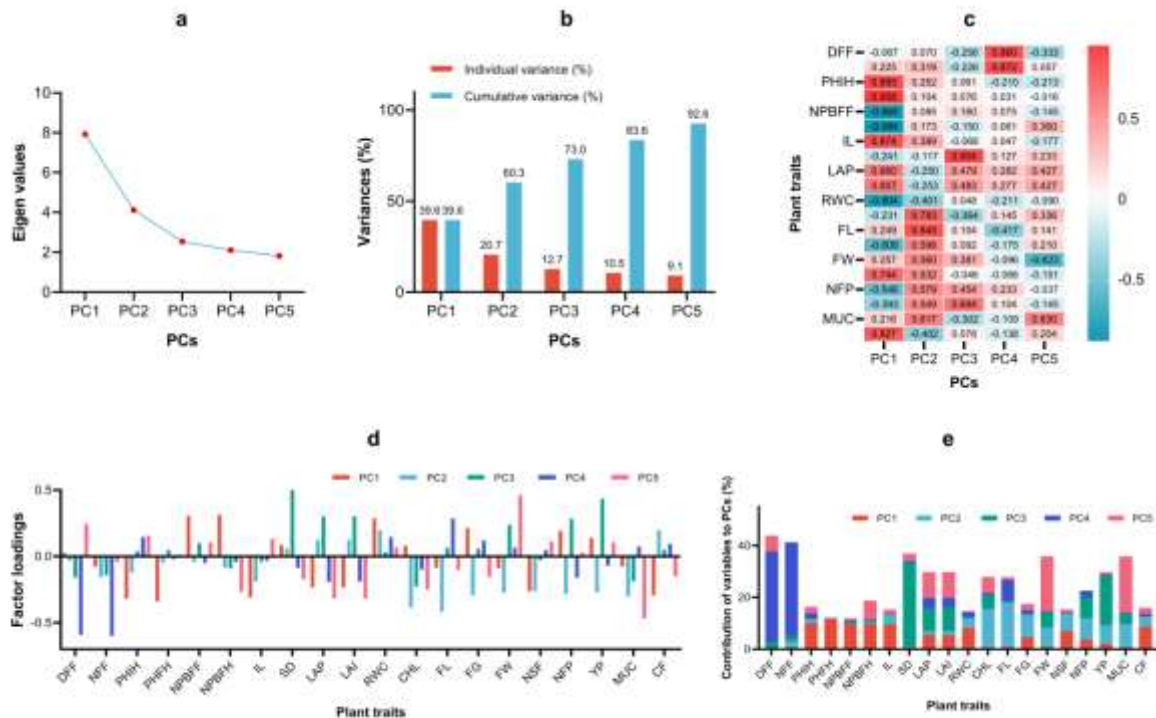
Fig. 2. PCA results showing the phenotypic variability in the okra plant traits under the influence of different plant growth regulators. a) Eigenvalue of PCs; b) Variances of PCs; c) Correlation between PCs and plant traits; d) Factor loadings of plant traits under PCs; e) Contribution of plant traits to PCs
