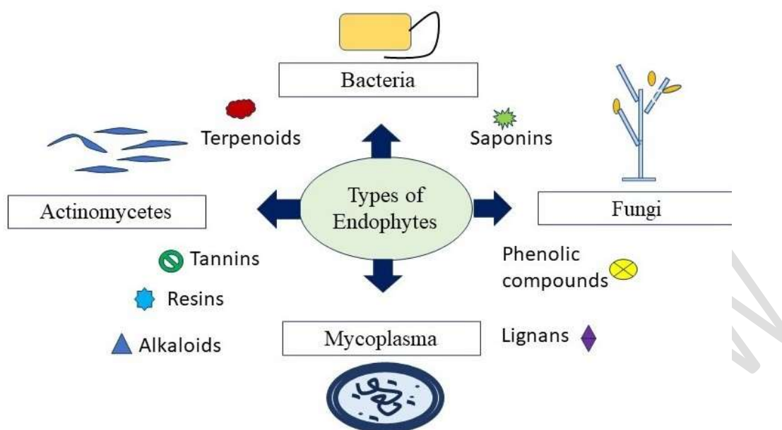
Fig 1: Different types of endophytes and the bioactive compounds produced
