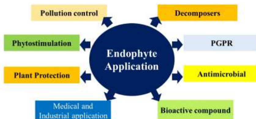
Fig 2: Application of endophytes in various fields
