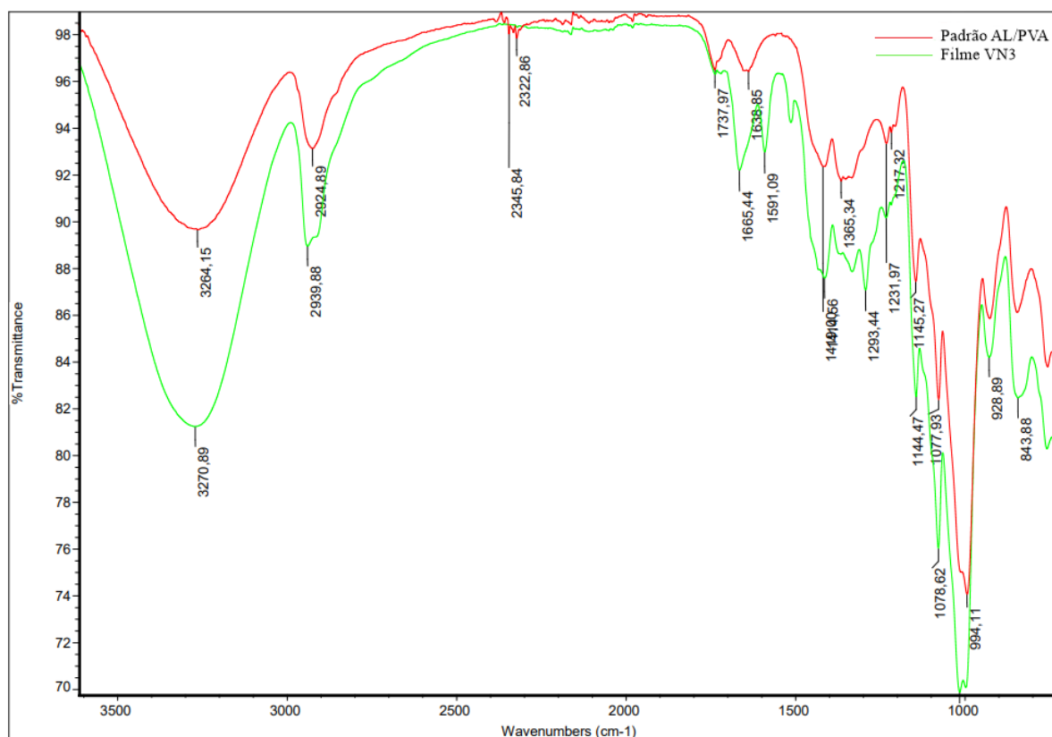
Figure 2. Fourier transform infrared spectrum of the Standard AL/PVA film and the VN film of 0.1% concentration of VN in the polymer matrix.
