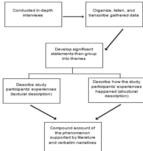
Figure 2. Analytical Framework
