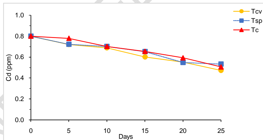
Fig. 10. Differences in the Cd conc. pre and post treatments
