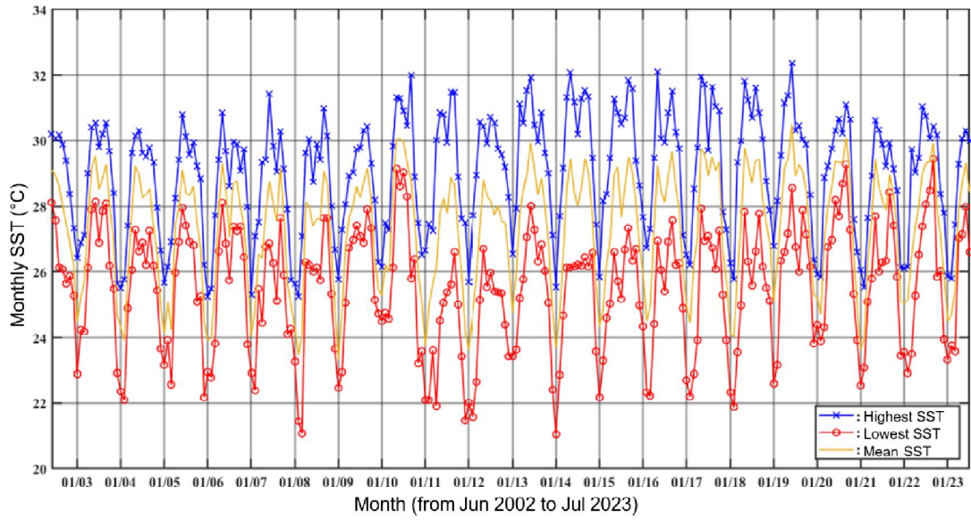
Figure 6. Changes in sea surface temperature (°C) according to monthly average over many years
