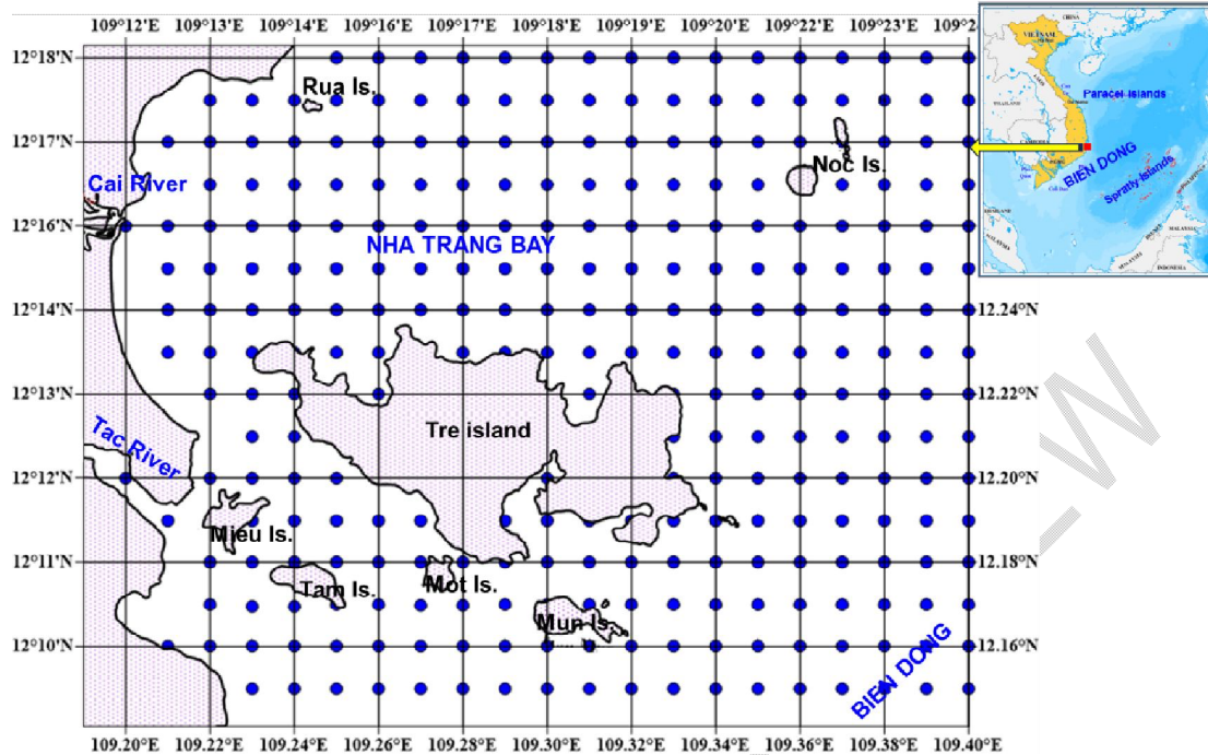
Figure 5. Extracted MUR SST point distribution for Nha Trang Bay
