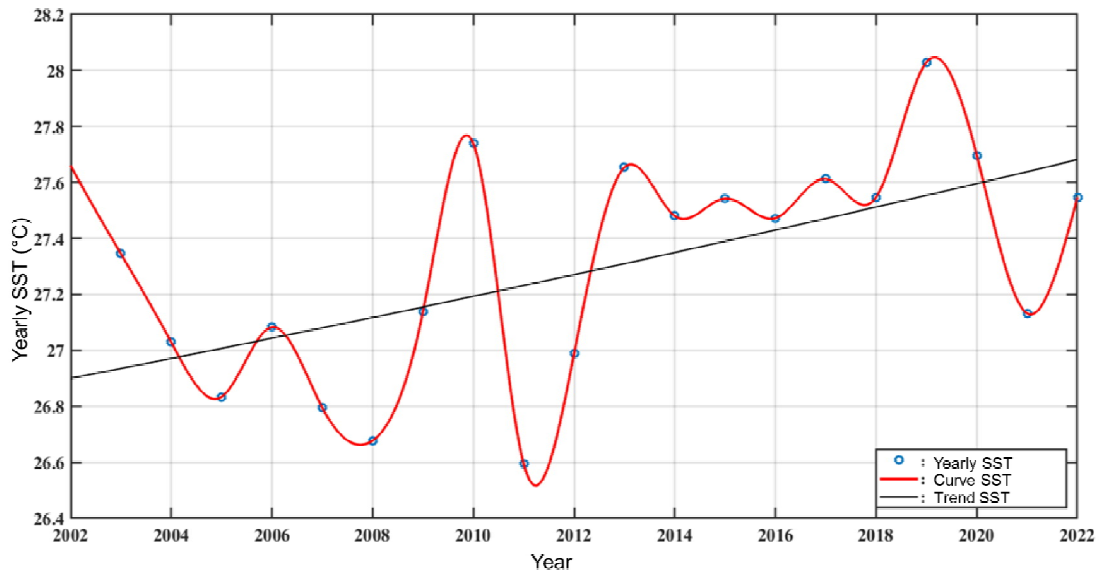
Figure 7. Average annual SST variation in the waters of Nha Trang Bay
