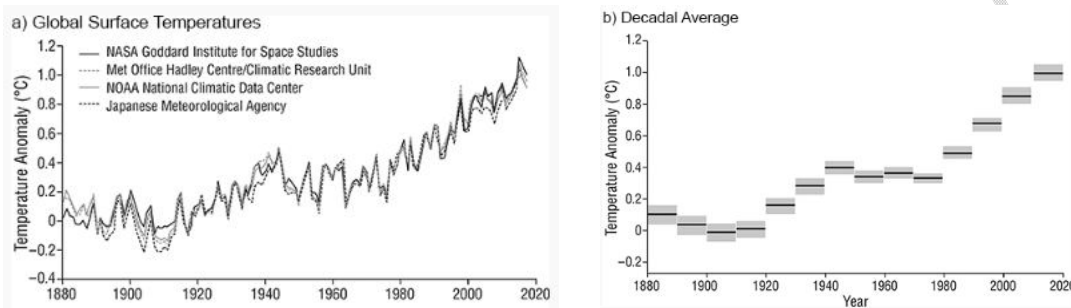
Figure 1. Change in Earth's surface temperature over the past 150 years[10]
