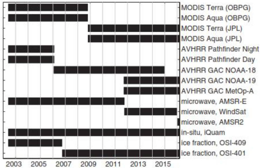
Figure 4. Input data sets used by Version 4.1 of the MUR SST analysis [21]
