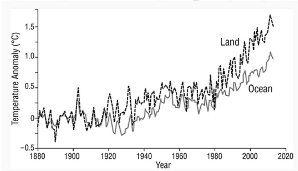
Figure 2. Land and ocean temperatures since 1880[10]
