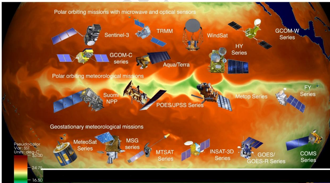
Figure 3. Major satellites contributing to the SST dataset [12]
