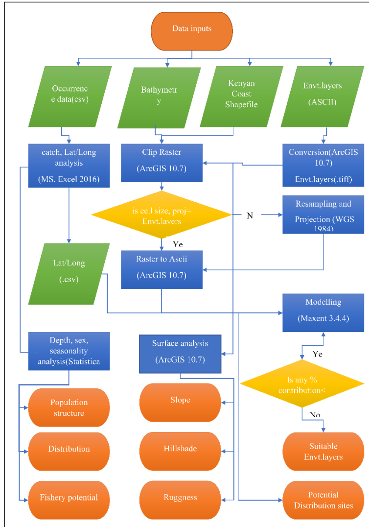
Fig. 1. The methodology of determining the population structure and species distribution modelling.
