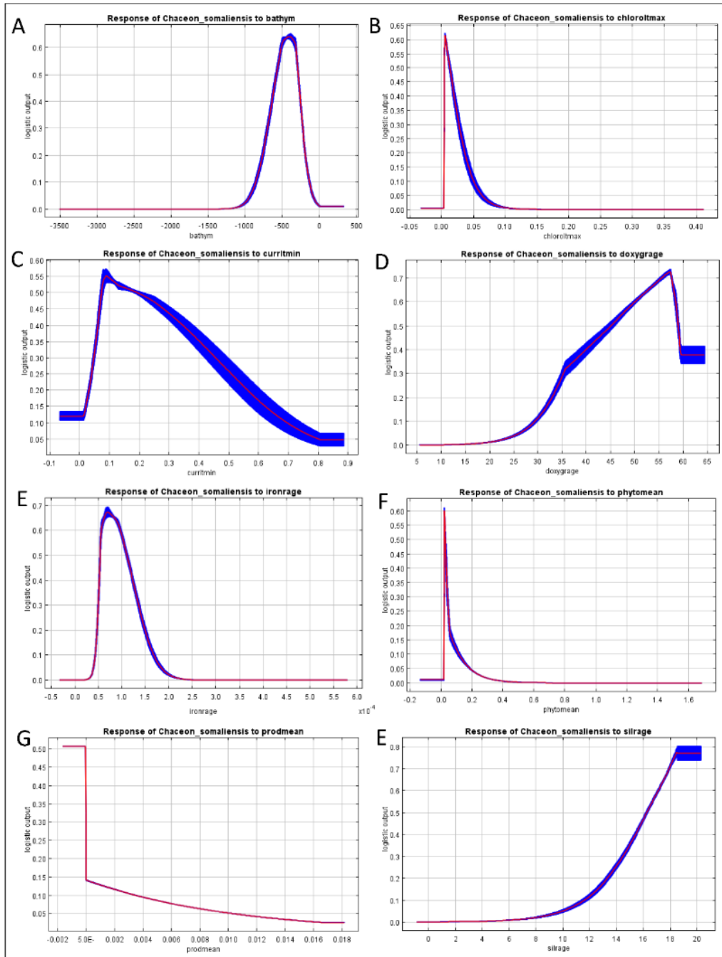
Fig. 6. The Chaceon somaliensis response curves for the environmental predictors.
