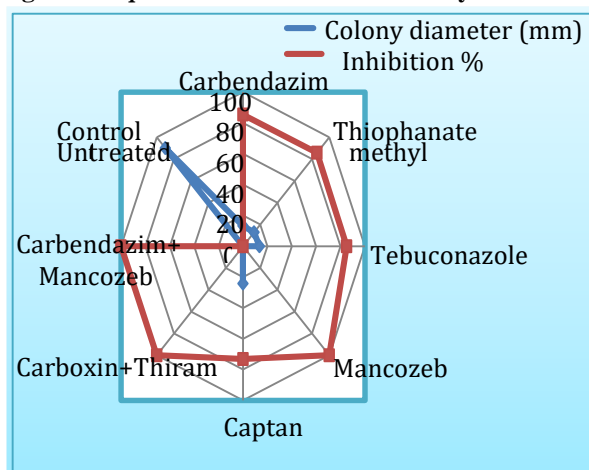
Fig. 1 C. In vitro efficacy of various fungicides against Alternaria alternata associated with soybean seeds
