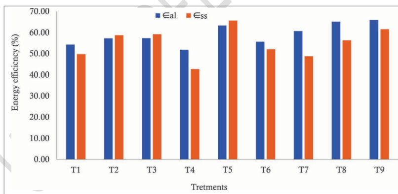
Figure 2. Effect of applied voltages (100 V) and different electrodes material on heat conversion efficiency
