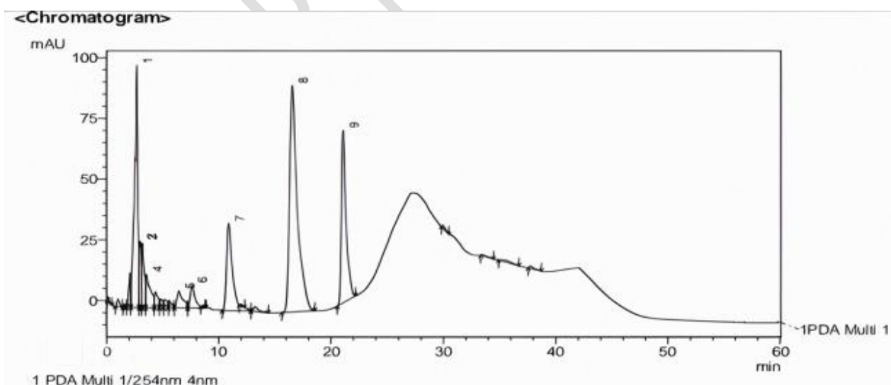
Figure 5: HPLC Chromatogram Resulting from the Analysis of Distilled Water Crude Leaves Extract of Anthocleista djalonensis at 254 nm Absorbance.
