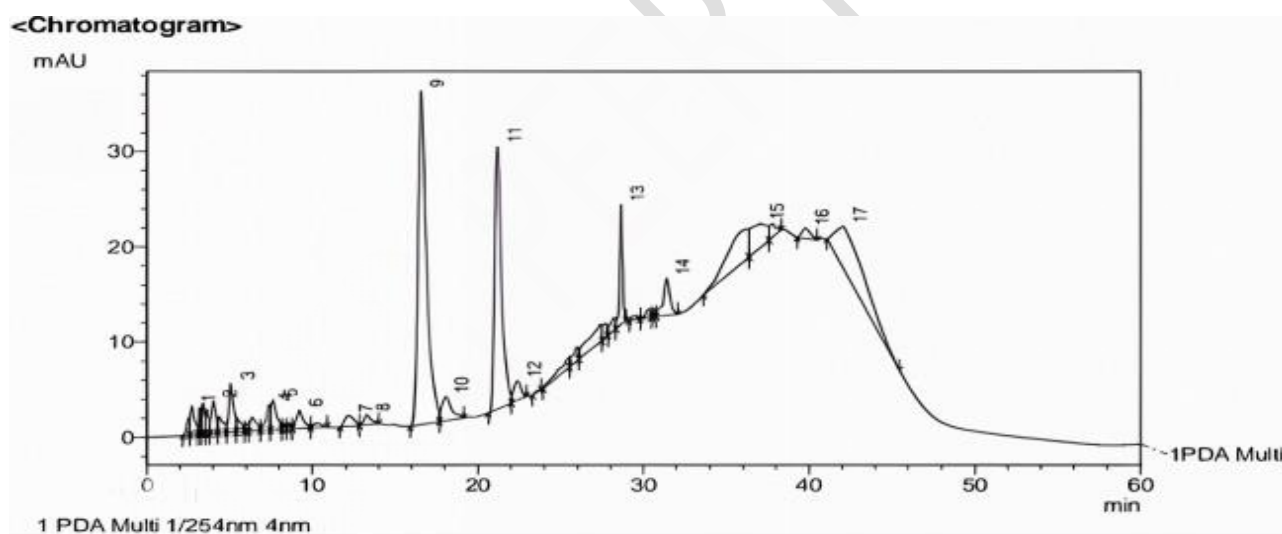
Figure 3: HPLC Chromatogram Resulting from the Analysis of Ethanol Crude Leaves Extract of Anthocleista djalonenis at 254 nm Absorbance.
