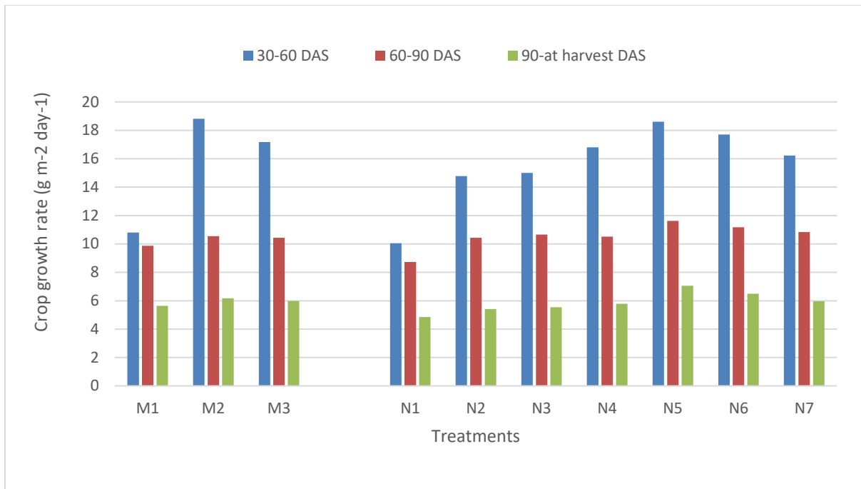
Fig. 1b. Effect of different crop establishment methods and nitrogen levels on crop growth rate ( \text{g m}^{-2} \text{ day}^{-1} ) of rice during 2023
