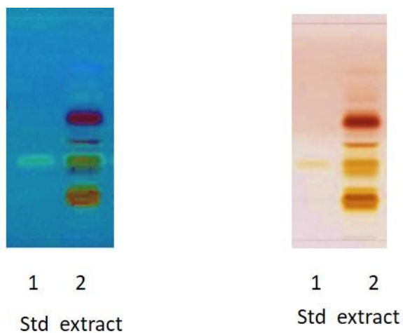
Figure 1. HPTLC analysis
