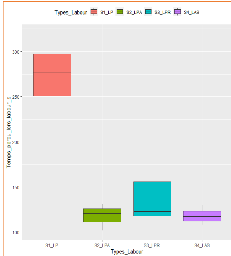
Fig 9: Boxplot of time lost (s) during plowing
