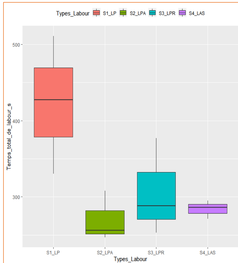
Fig 11: Boxplot of the total plowing time (s) according to the different trajectories for motorized plowing
