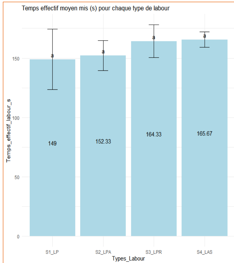
Fig 8: Comparison of the average effective time (s) spent on plowing with the different trajectories
