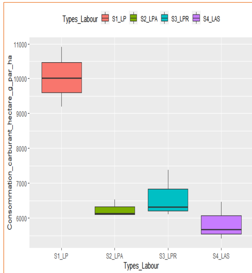
Fig 13: Boxplots of fuel consumption per hectare (g/ha)
