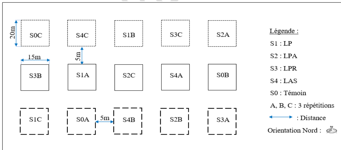
Fig 4: Randomized complete block experimental design
