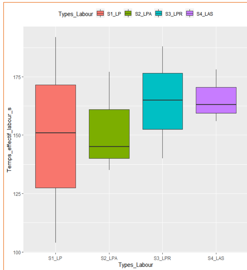
Fig 7: Boxplots of the effective time (s) according to the different trajectories for motorized plowing
