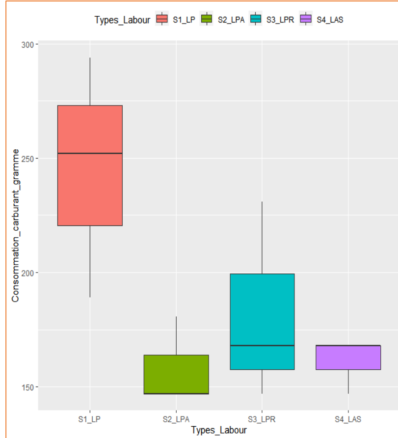
Fig 5: Boxplot of fuel consumption (g) of trajectories for motorized plowing
