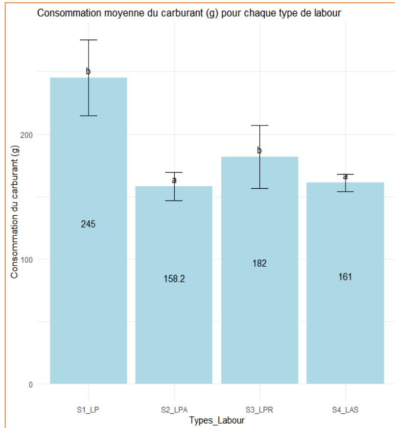
Fig 6: Comparison of fuel consumption (g) of trajectories for motorized plowing
