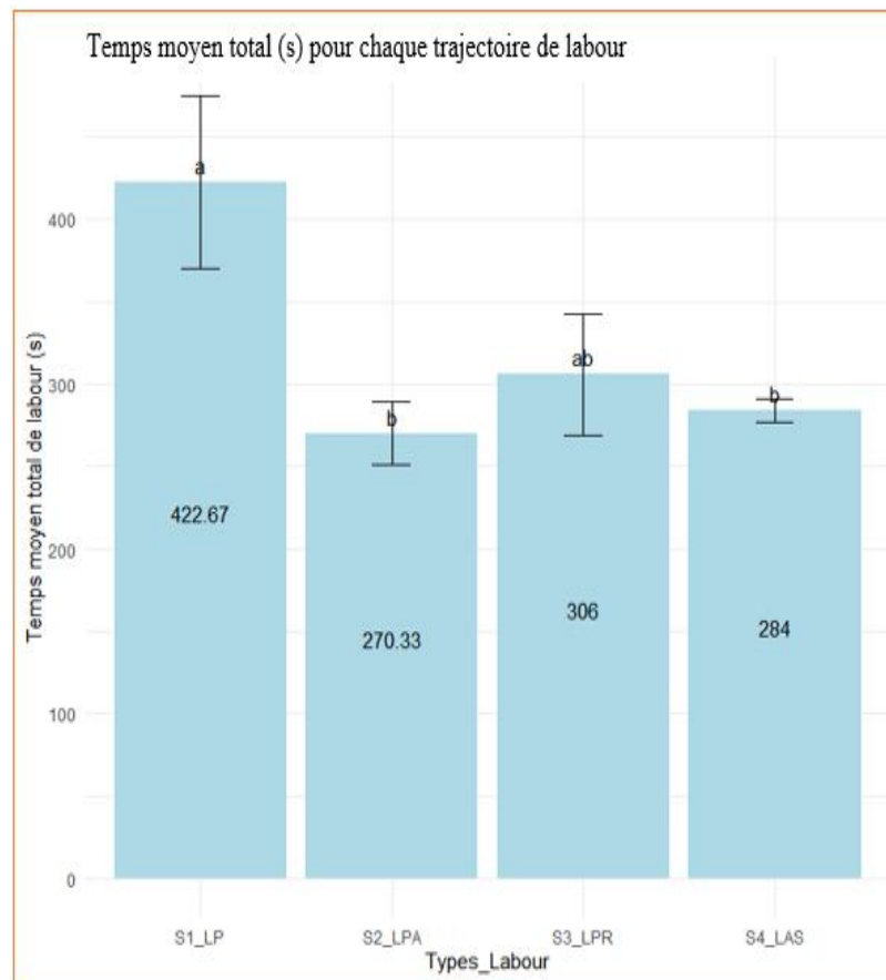
Fig 12: Comparison of the total average plowing time (s) according to the different trajectories for motorized plowing
