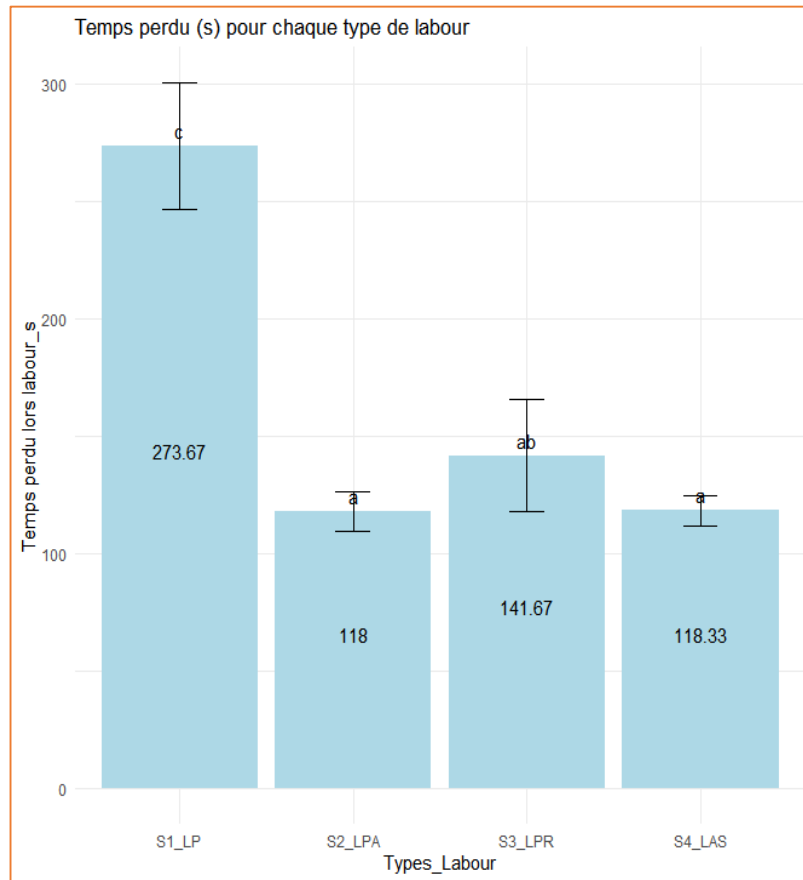
Fig 10: Comparison of the average time lost (s) when executing trajectories for motorized plowing
