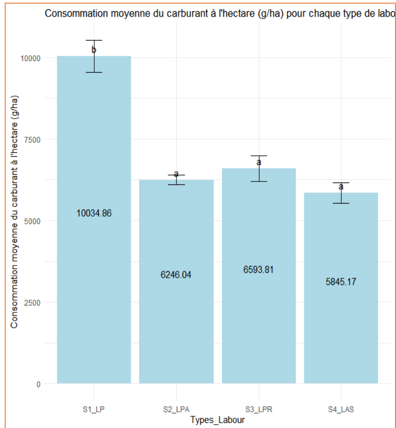
Fig 14: Average fuel consumption per hectare (g/ha)
