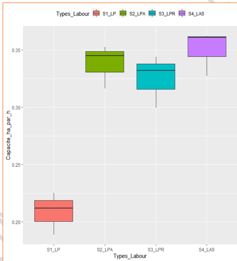
Fig 17: Boxplot of field capacity (ha/h) per trajectory for motorized plowing
