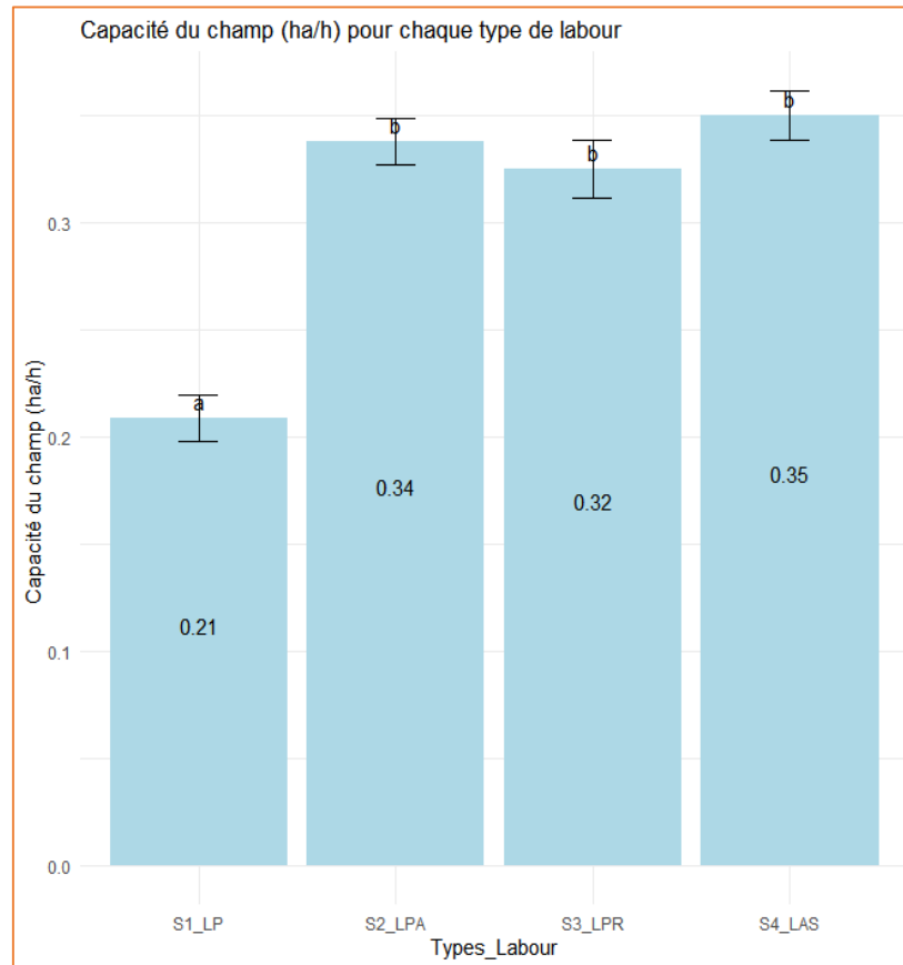
Fig 18: Comparison of average capacity (ha/h) per trajectory for motorized plowings
