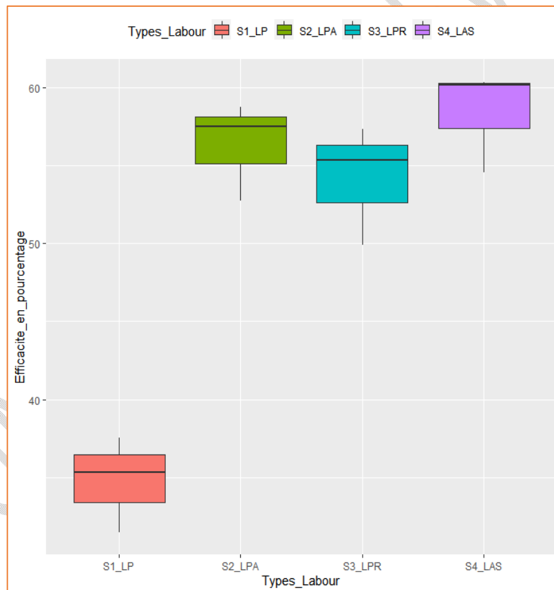
Fig 15: Boxplot of field temporal efficiency (%) by trajectory for motorized plowing
