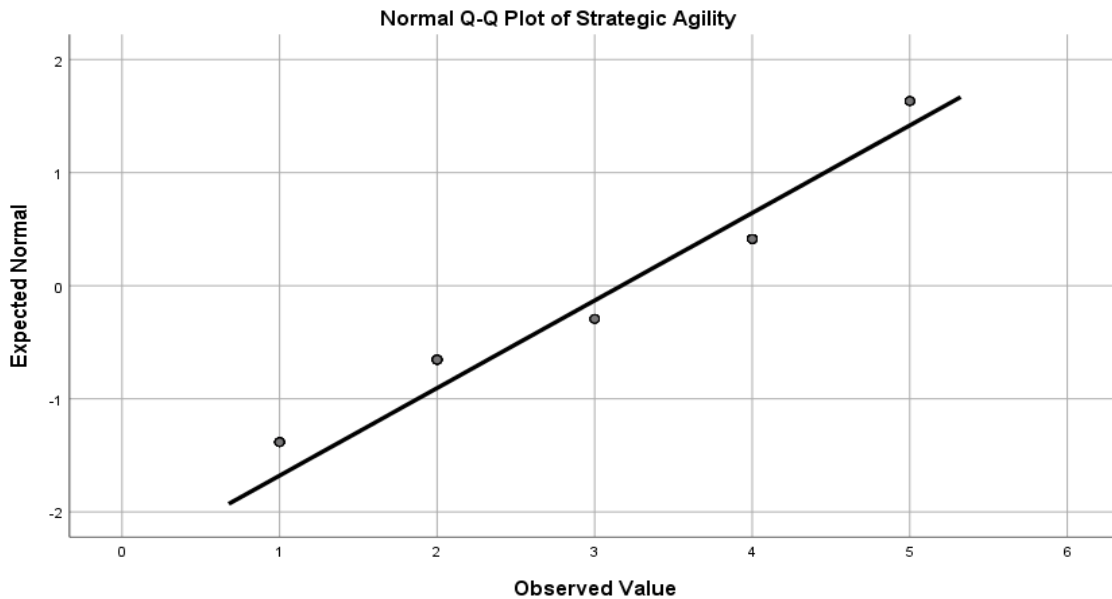
Figure 1: Normality test for Strategic Risk Adaptability
