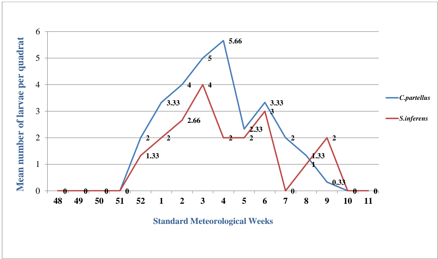
Fig. 1: Population dynamics of C. partellus and S. inferens on sorghum in relation to weather parameters during rabi season 2020-21
