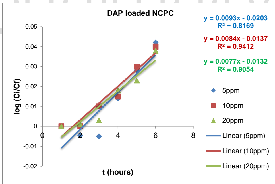
Fig.3. Plot of first order kinetic equation for P sorption
