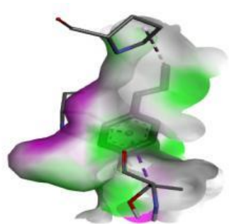
Anethole 3D
