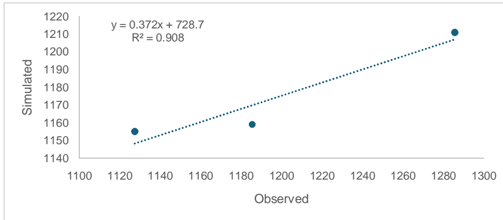
Fig. 7. Simulated and Observed grain yield (kg/h) during validation
