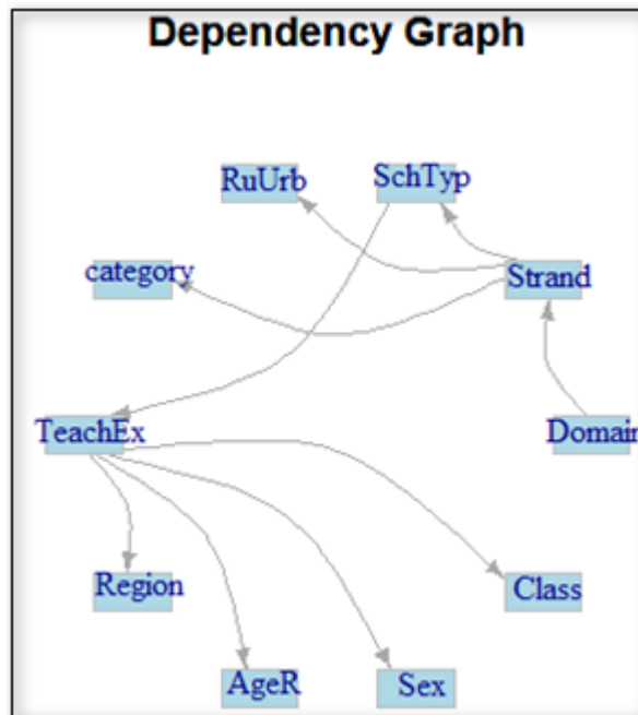
Figure 8. Dependency Relationships
