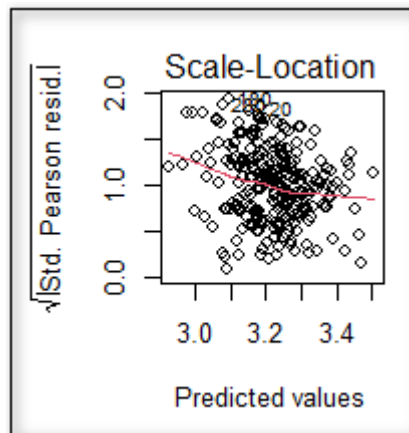
Figure 3. Scale-Location Plot
