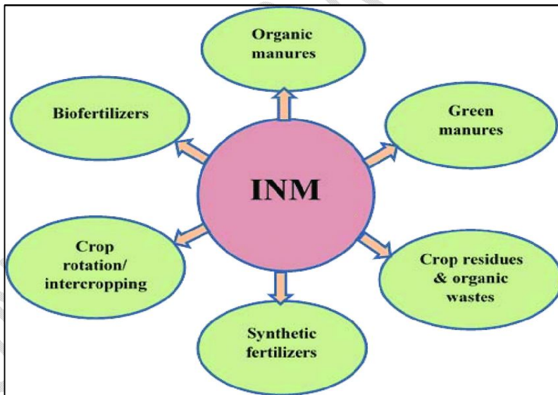
Fig. 1: Various components of an integrated nutrient management
