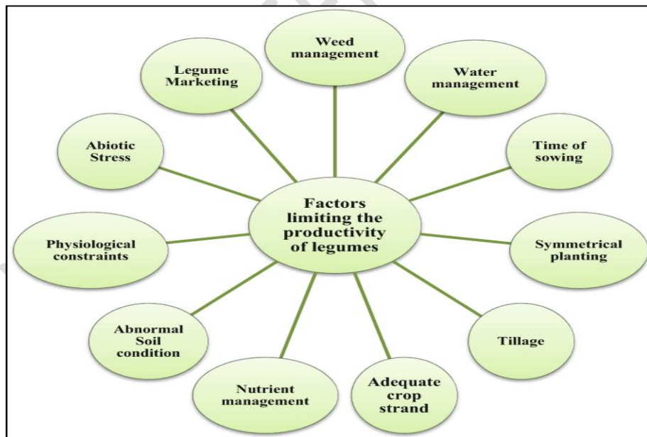
Fig. 2: Factors limiting the productivity of legumes
