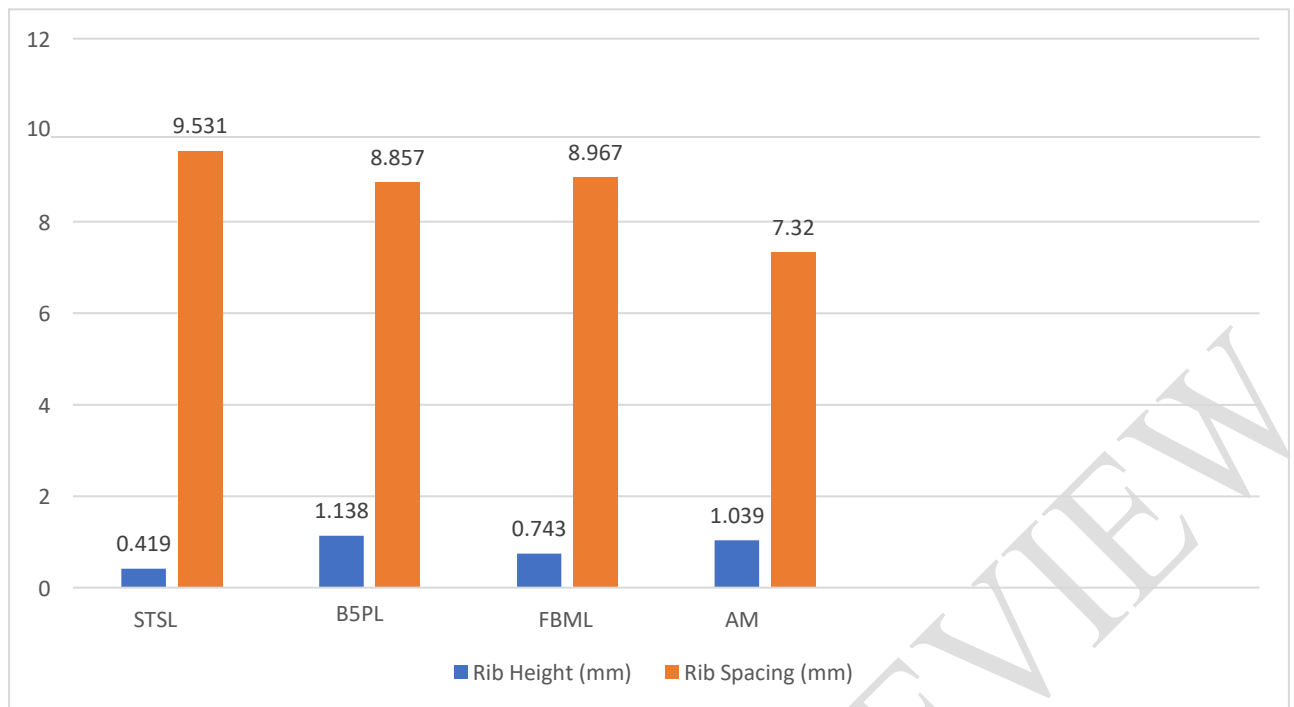
Fig. 6: Rib Height and Rib Spacing of 12mm Reinforcing bars
