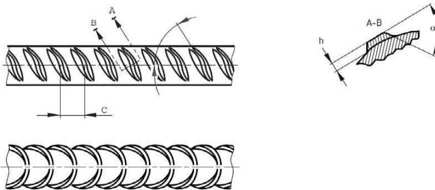
Fig 1: Illustration of Rib Geometry for Ribbed Bars.
