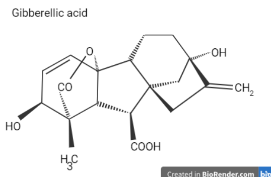
Fig 1 Chemical structure of Gibberellic acid
