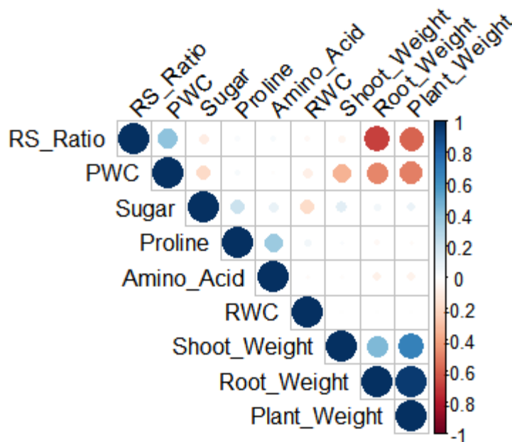
Fig. 6. Pearson correlation matrix among evaluated variables.
