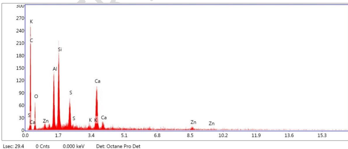
Figure 4. EDAX Analysis of untreated reclaimed rubber
