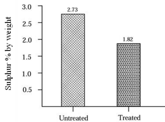
Figure 7(a). Sulphur reduction of reclaimed rubber treated for 1 hour with Benzoyl Peroxide in Toluene.
