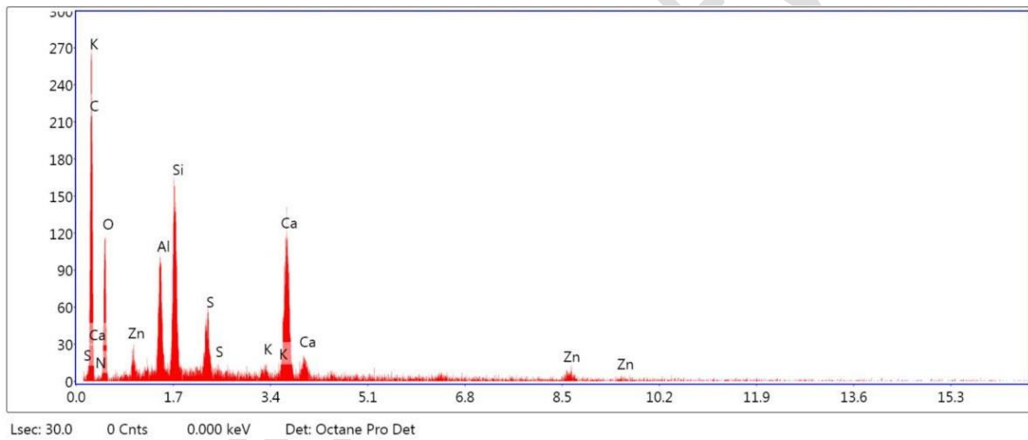
Figure 5(a). EDAX Analysis of sample treated with o-Xylene & BPO for 1 hour
