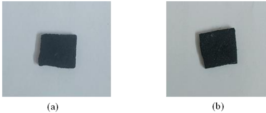
Figure 3. Devulcanized rubber obtained using (a) o-Xylene & (b) Toluene after drying for 10 mins at 80°C
