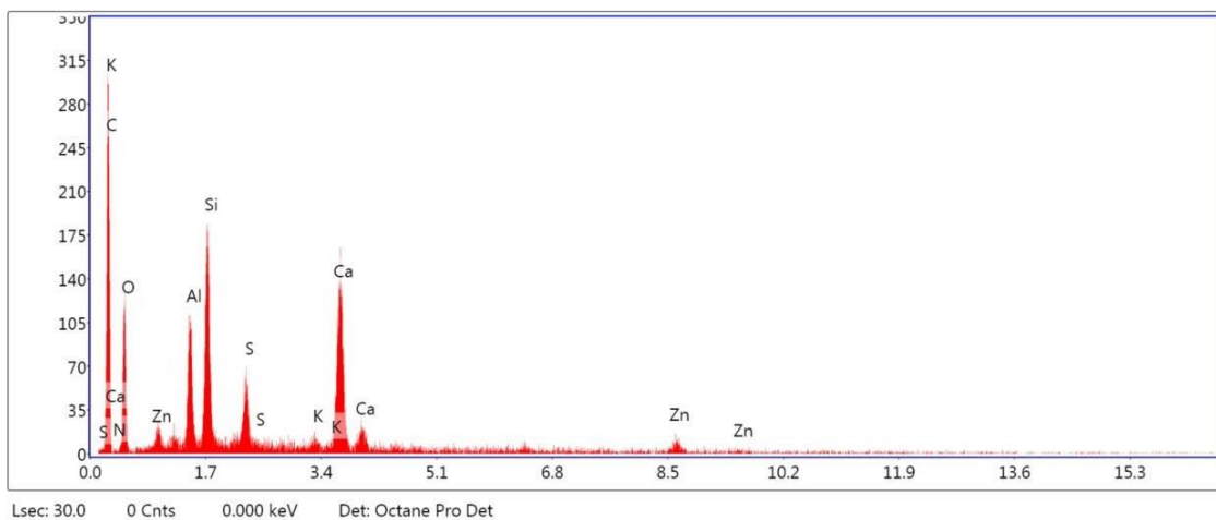
Figure 6(a). EDAX Analysis of sample treated with o-Xylene & BPO for 1.5 hours
