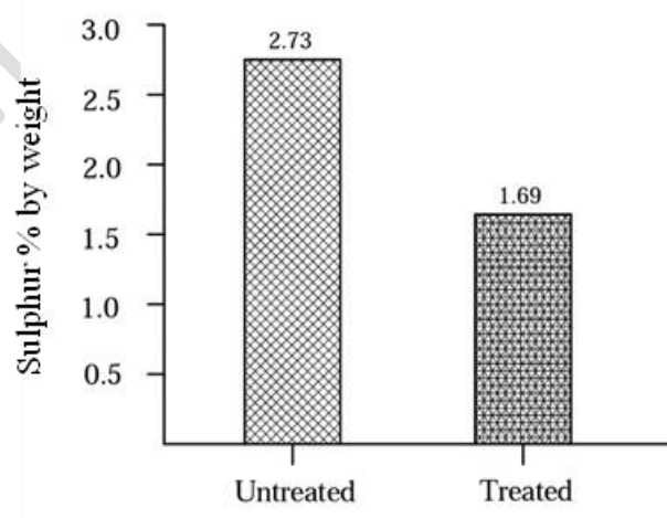
Figure 7(b). Sulphur reduction of reclaimed rubber treated for 1.5 hours with Benzoyl Peroxide in Toluene.
