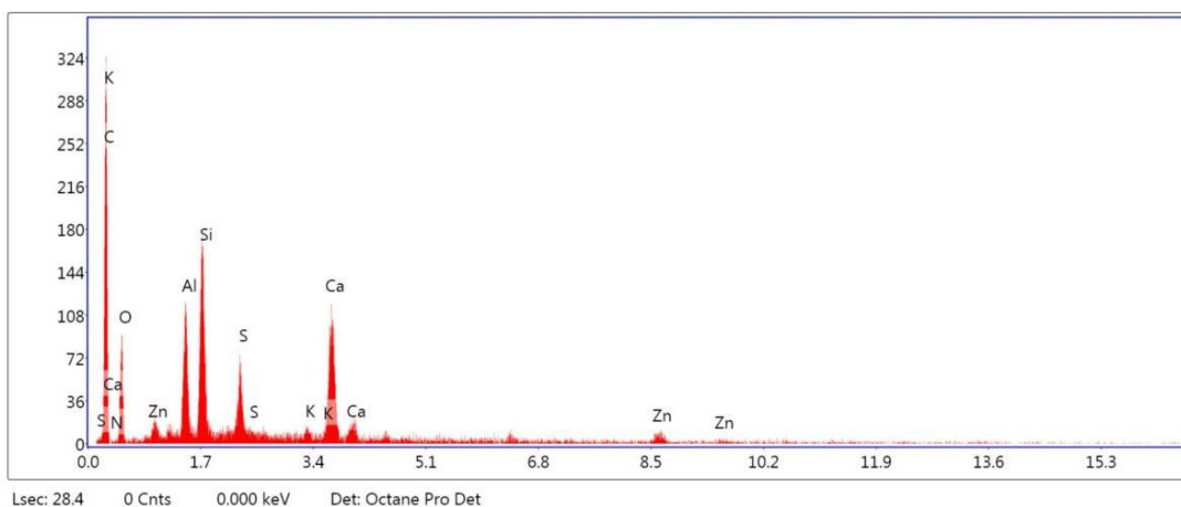
Figure 5(b). EDAX Analysis of sample treated with Toluene & BPO for 1 hour
