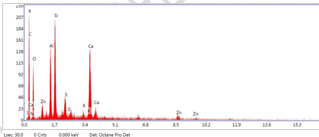
Figure 6(b). EDAX Analysis of sample treated with Toluene & BPO for 1.5 hours
