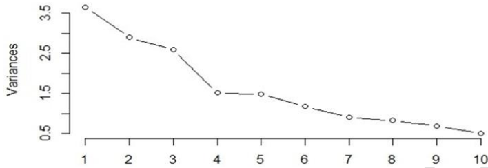
Fig 1: Scree Plot
