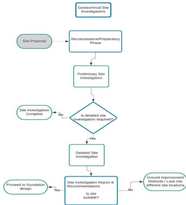
Figure 1: Stages of a geotechnical site investigation
