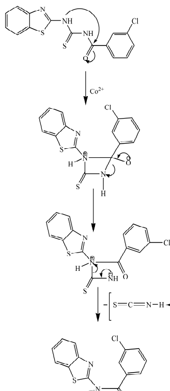
Scheme 2. Proposed mechanism for the formation of (2)
