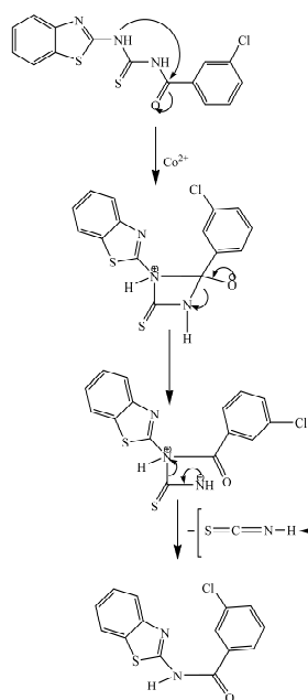
Scheme 2. Proposed mechanism for the formation of (2)
