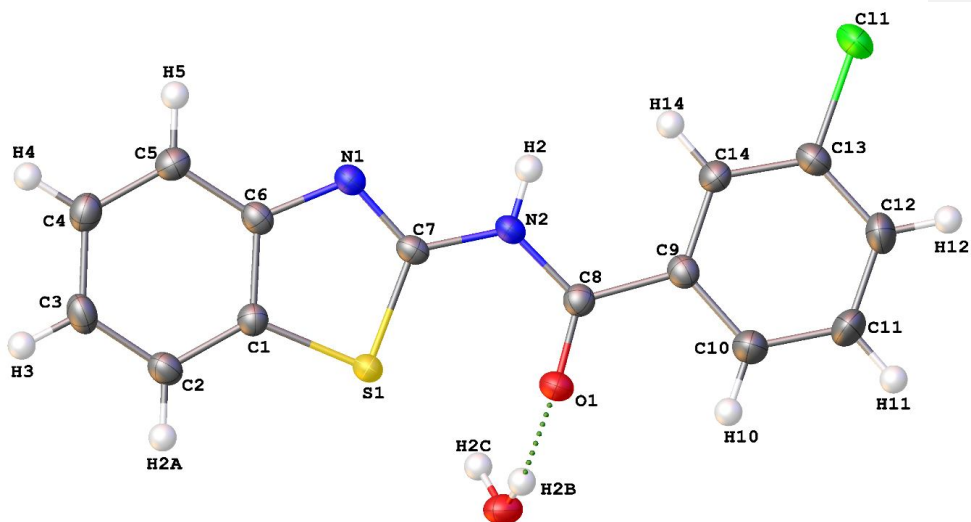
Figure 1. ORTEP plot (30% probability ellipsoids) showing the structure of (2).
