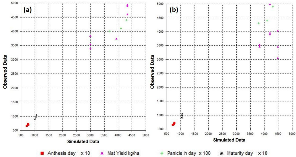
Figure 1: The scatterplot showing observed and simulated values of anthesis, panicle initiation, maturity day and yield during (a) calibration and (b) validation
