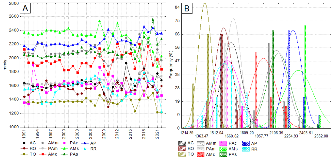
Fig. 2. A) Average annual distribution of rainfall and B) Class frequency histogram for the seven states in the North region of Brazil. Legend: m = southern; c = central and s = northern zone.
