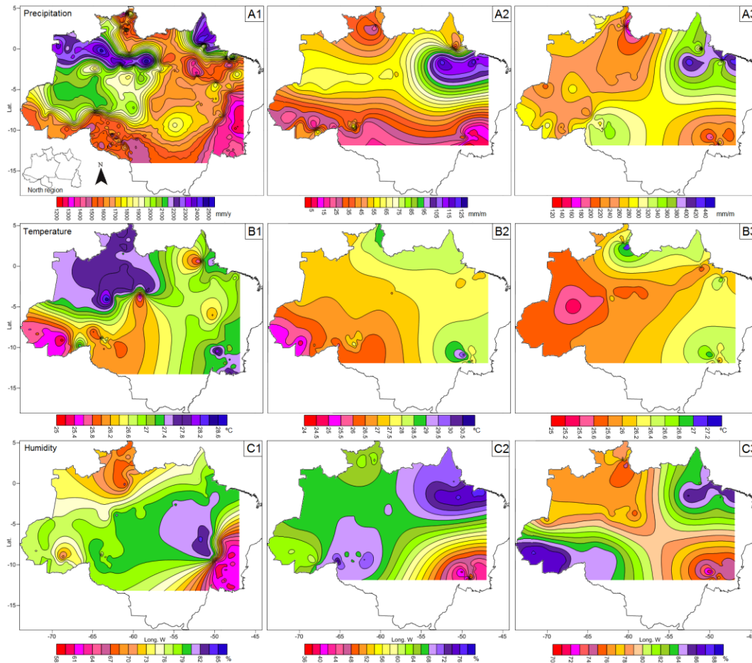
Fig. 5. Spatio-temporal variation of the A) precipitation, B) temperature and C) relative humidity of air for annual (1); drought (2); and rainy (3) seasonal periods by interpolation of data from meteorological stations, satellite estimates and conjunction of primary data from historical series from 1991 to 2022.
