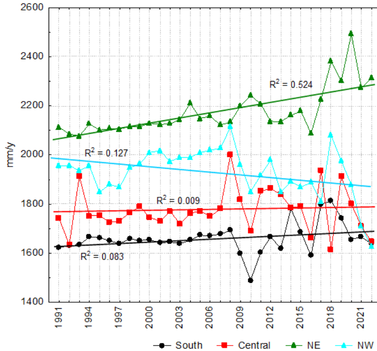
Fig. 4. Average annual rainfall per quadrant in the North region of Brazil for the historical series from 1991 to 2022.
