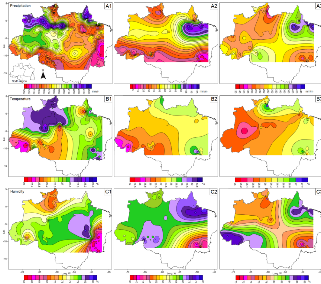
Fig. 5. Spatio-temporal variation of the A) precipitation, B) temperature and C) relative humidity of air for annual (1); drought (2); and rainy (3) seasonal periods by interpolation of data from meteorological stations, satellite estimates and conjunction of primary data from historical series from 1991 to 2022.
