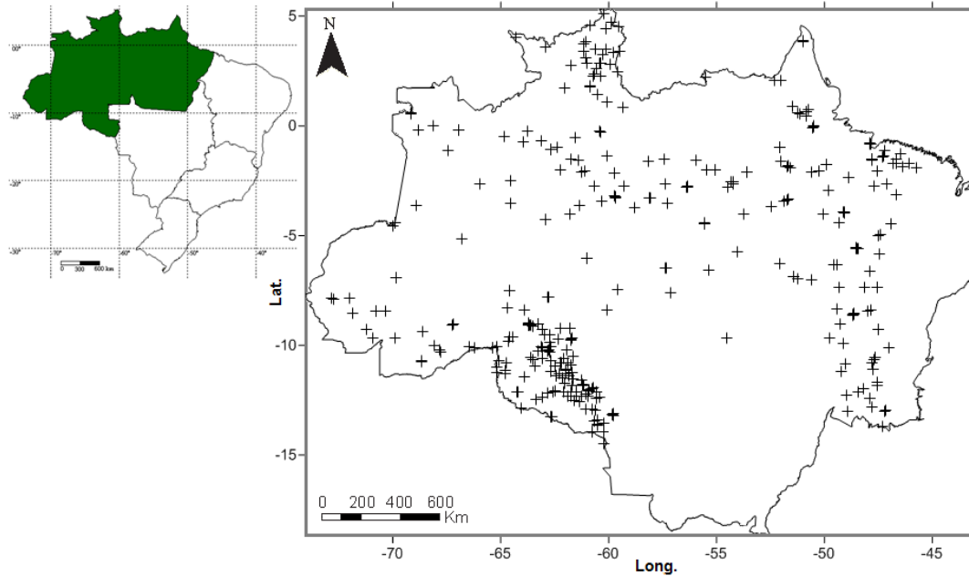
Fig. 1. Distribution of conventional and automatic meteorological stations consulted for the application of the rainfall model in the Amazon – North Region of Brazil (Legal Amazonian Map generated in ArcGis® 9.3 ©2008).
