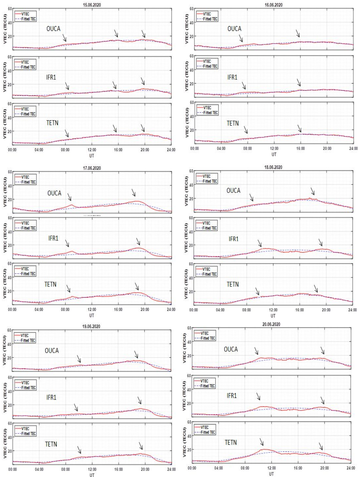
Figure5: VTEC and VTEC_{fit} against UT for OUCA-IFR1-TETN receiver array between 15 th -20 th June 2020
