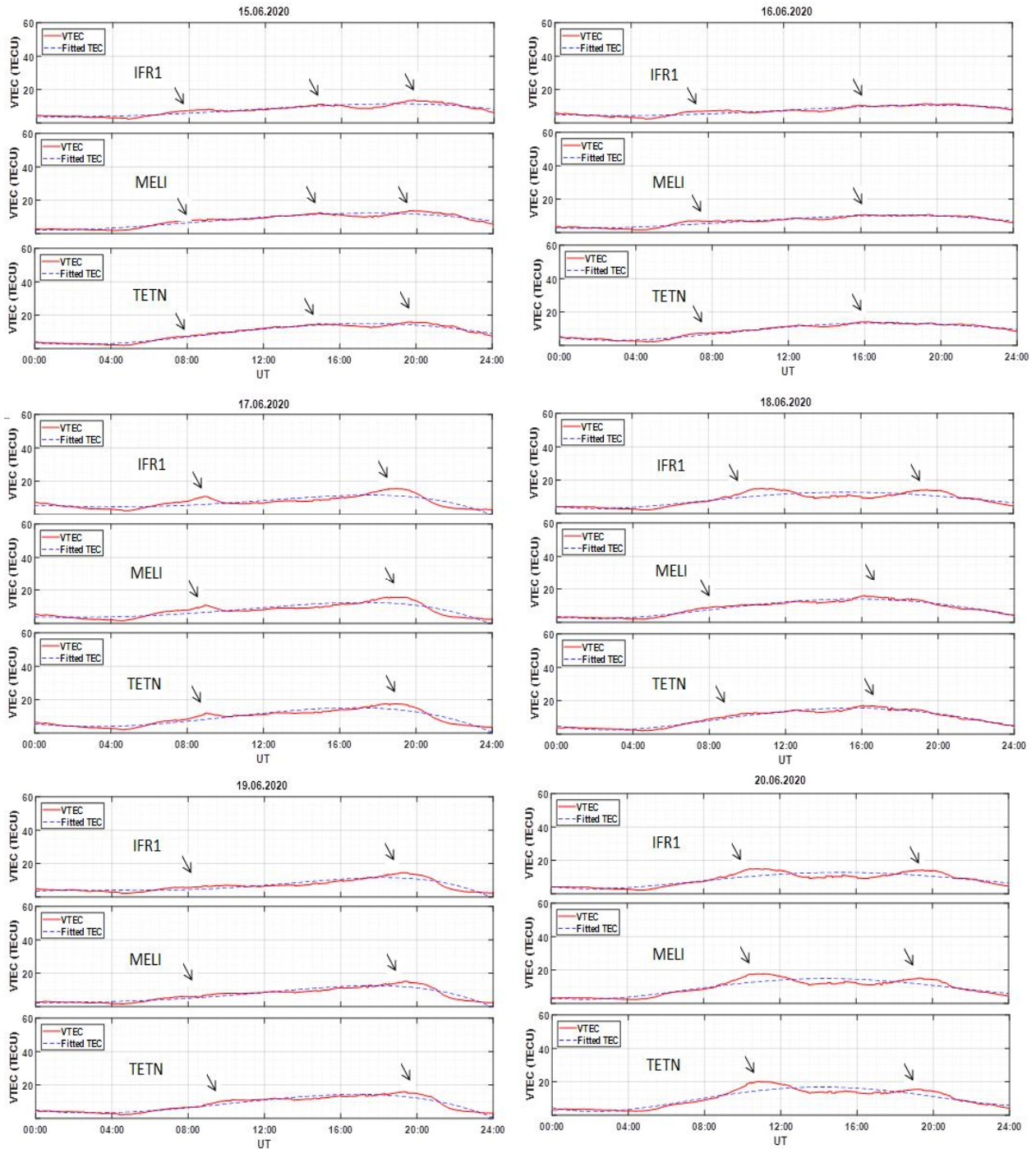
Figure7: VTEC and VTEC_{fit} against UT for IFR1-MELI-TETN receiver array between 15 th -20 th June 2020
