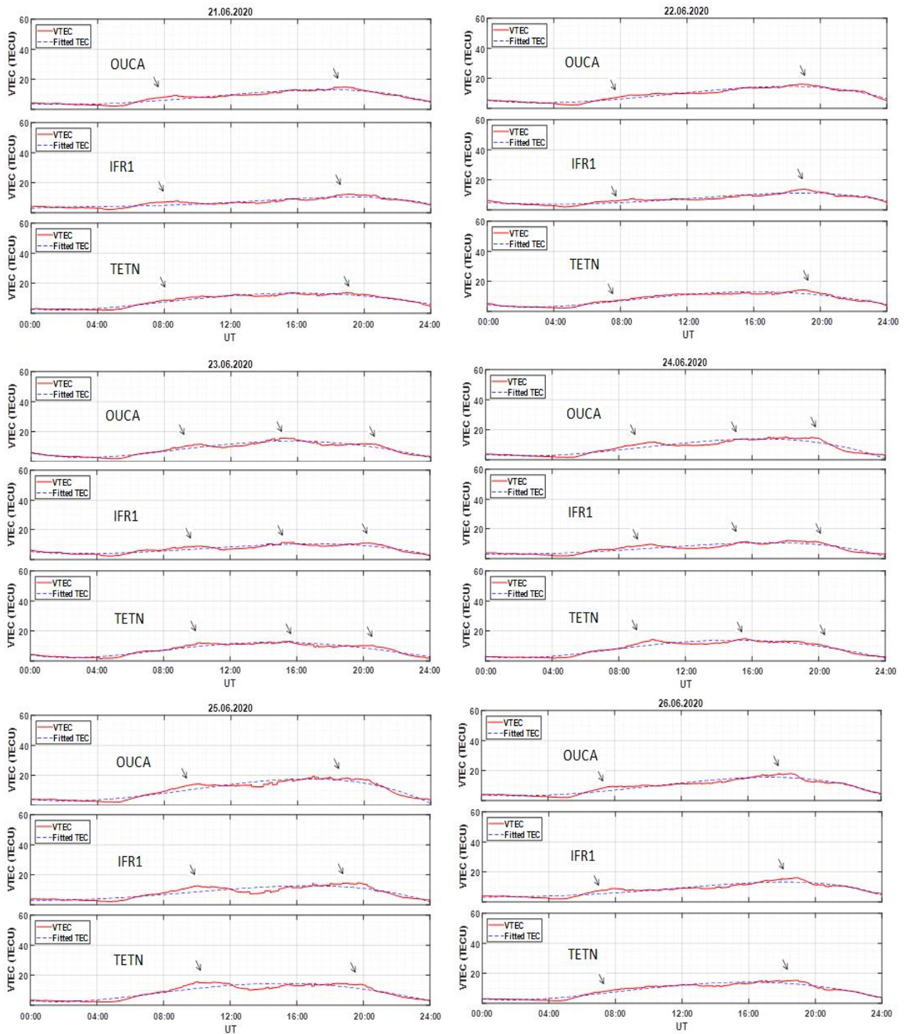
Figure 6: VTEC and VTEC_{fit} against UT for OUCA-IFR1-TETN receiver array between 21 st -26 th June 2020
