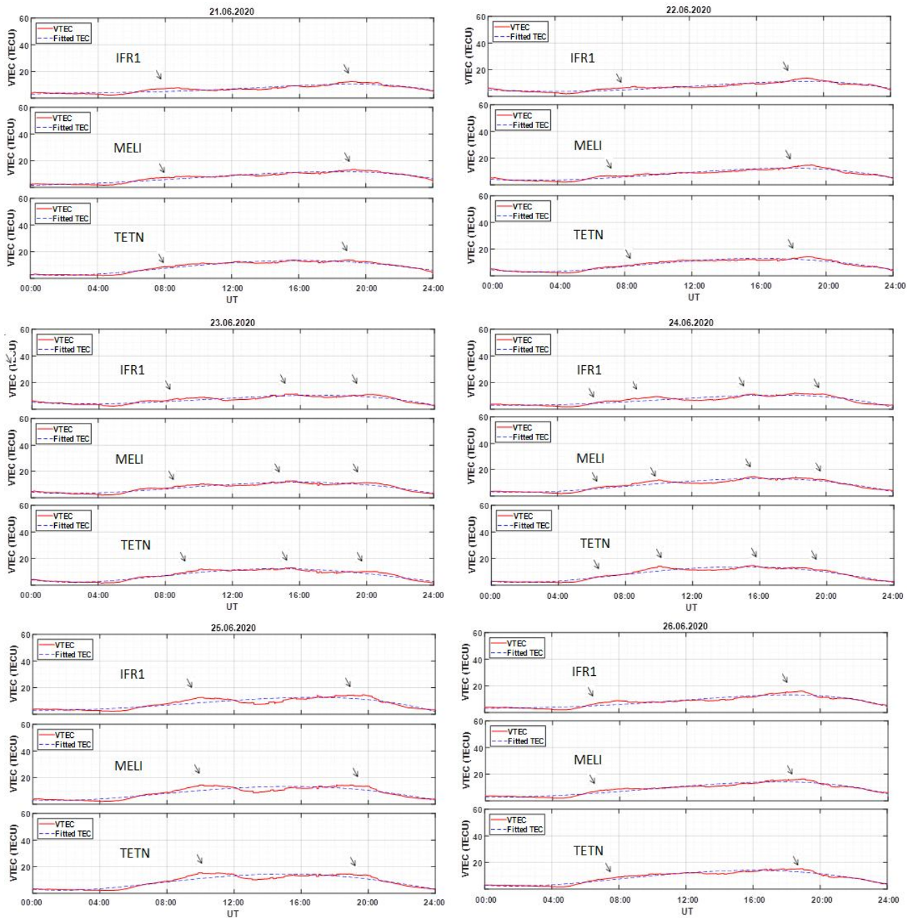
Figure 8: VTEC and VTEC_{fit} against UT for IFR1-MELI-TETN receiver array between 21 st -26 th June 2020
