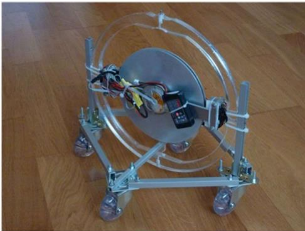
Figure 5. Terrestrial Prototype II with rotating wheels, which allowed its direction control, with results similar to those of the submarine. 5
