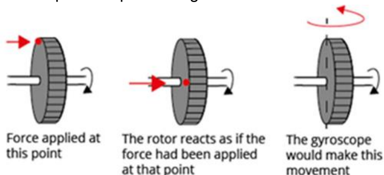
Figure 4. The precession in rotational dynamics is generated when a force is applied to a rotating body, forcing it to perform a new turn, on a new axis. The mobile's response is not that new turn, but it reacts as if the force had been applied at another point, which forces it to perform an orbital movement, as this
