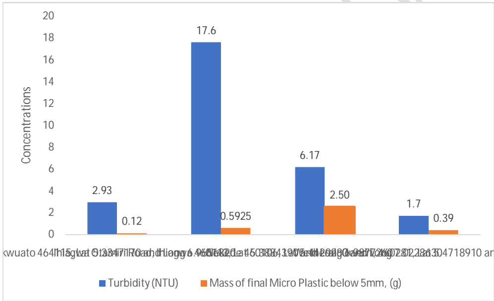
Fig 7: Correlation between Turbidity of Otammiri River and the microplastics concentration of Otammiri River
