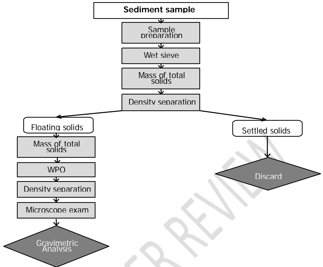
Fig 3: Flow diagram for the analysis of microplastics in sediment samples (Miller et al. , 2021).
