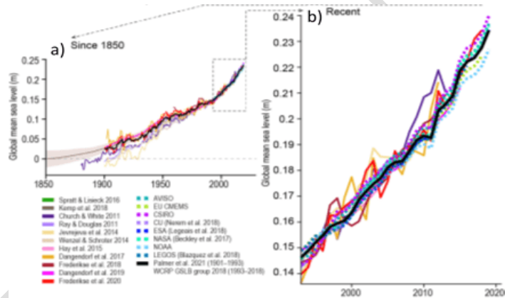
Fig. 2 Changes in global mean sea level a) Estimates based on tide gauges and altimeters since 1850 b) The most recent recording period [4].
