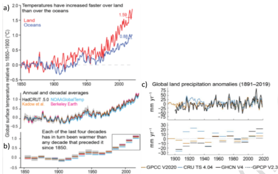
Fig. 1 Evolution of the Earth's surface temperature. (a) Temperature from instrumental data in the period 1850-2020, multi-product annual mean time series assessed for ocean temperature (blue line) and land temperature (red line) and indicating warming up to the last 10 years; and (b) annual and decadal averages for GMST data. Gray shading shows the uncertainty associated with the estimate [3]; (c) Changes in observed precipitation. Annual and decadal mean time series from 1891 to date relative to climatology 1981-2010 [4].
