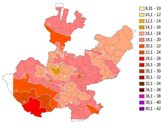
Figure 15 Average temperatures of the State of Jalisco according to the Climatological Normals of the period 1981-2010.
