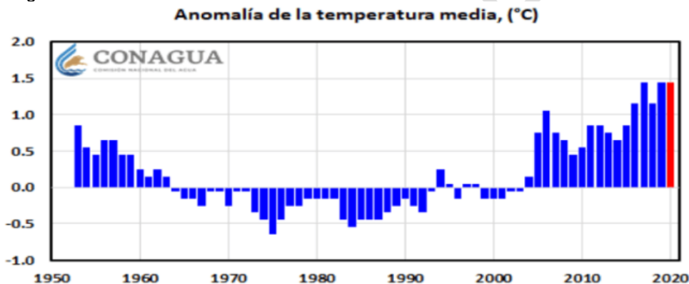
Fig. 4 Annual mean temperature anomaly (°C), the red bar corresponds to the estimated national anomaly in 2020. Based on measurements since 1953 by the National Weather Service [5].
