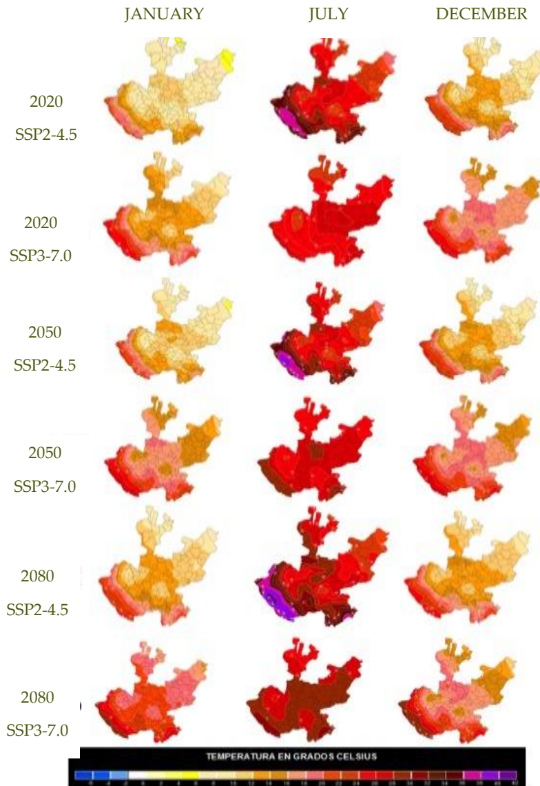
Fig. 17 Temperature projections using the PRECIS model for the months of January, July and December under the IPCC SSP2-4.5 and SSP3-7.0 scenarios; by 2020-2080.
