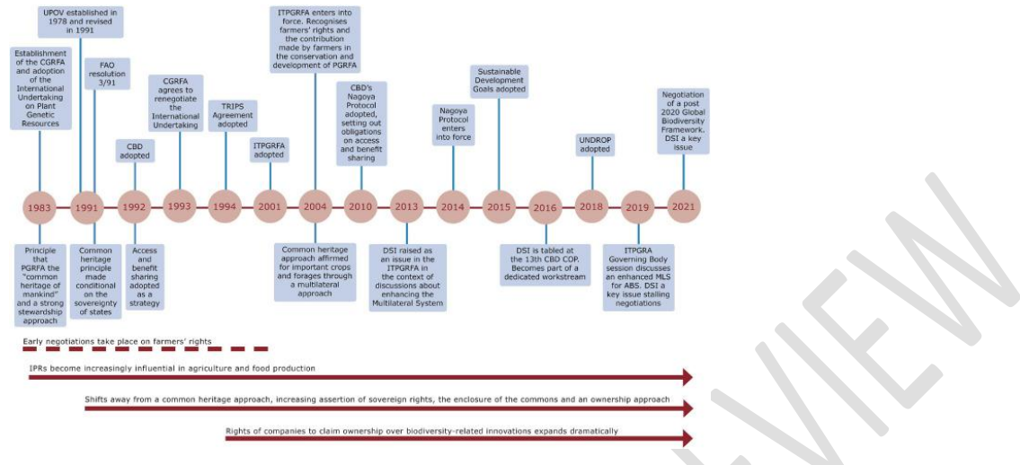
Fig 1. ABS framework
