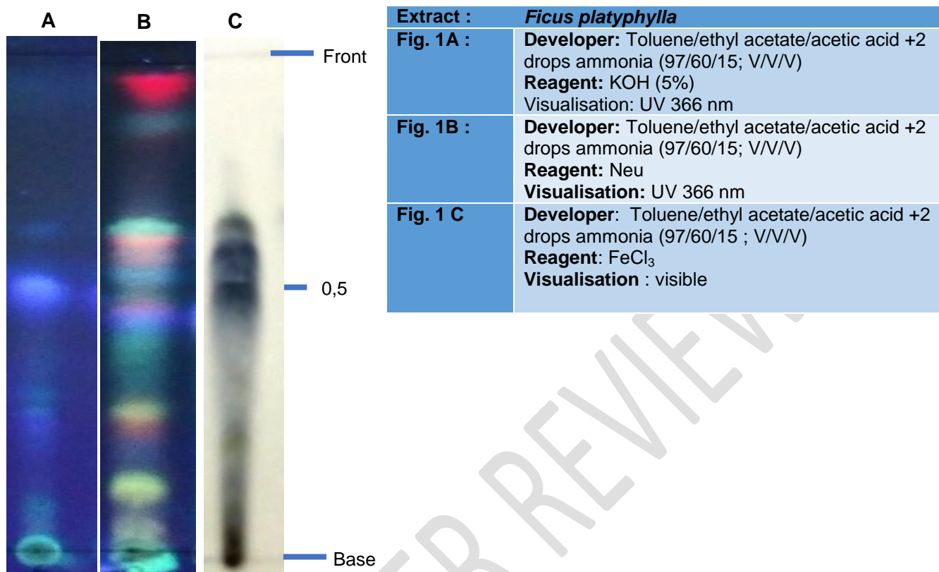
Fig. 1. TLC of F. platyphylla bark extract
