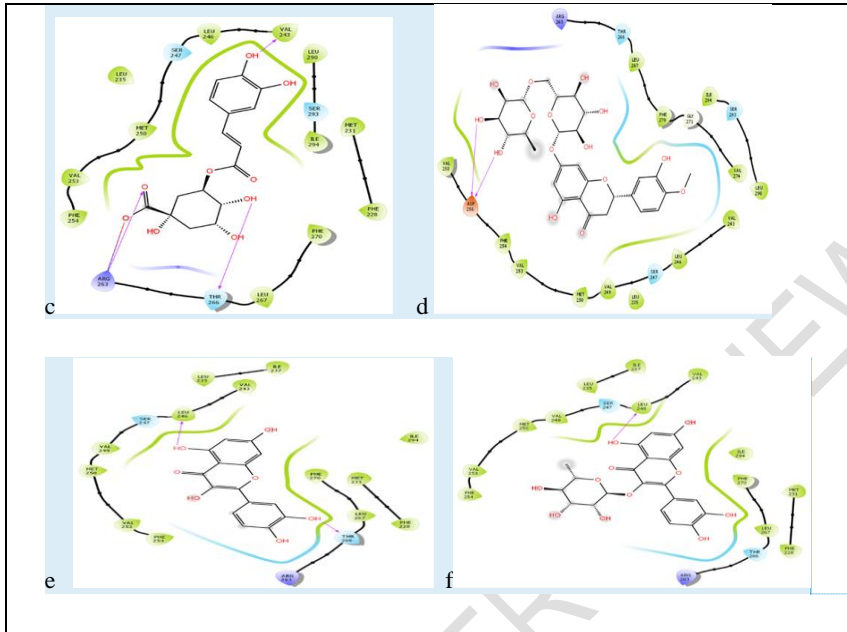
Figure 1: 2D Molecular contacts profiling of docked compounds with amino acid residues at the active site of Mcl-1 (a) 6u6f ligand (b) Apigenin (c) Chlorogenic acid (d) Hesperidin (e) Quercetin (f) Quercitrin
