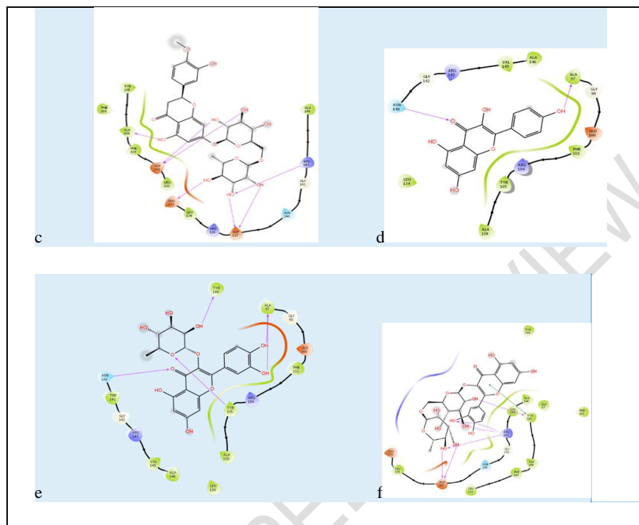
Figure 2: 2D molecular contacts profiling of docked compounds with amino acid residues at the active site of Bcl-xL: (a) 201Y ligand (b) Chlorogenic acid (c) Hesperidin (d) Kaempferol (e) Quercitrin (f) Rutin
