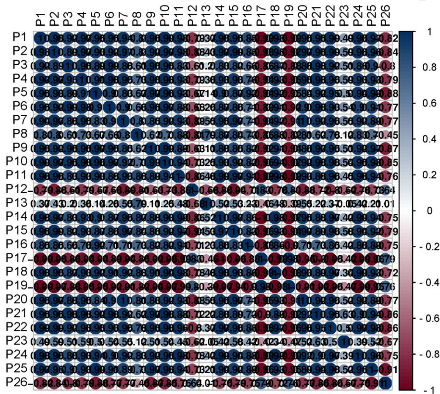
Figure4. Correlation matrix showed almost all characters positively significantly correlated with each other except siliqua length (P12), leaf osmotic potential (P17), electrolyte leakage (P19), and harvest index (P26).
