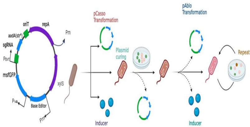
Figure 3: Graphical Representation of the pAbo-pCasso self-curing vector toolset for unconstrained cytidine and adenine base-editing in Gram-negative bacteria.
