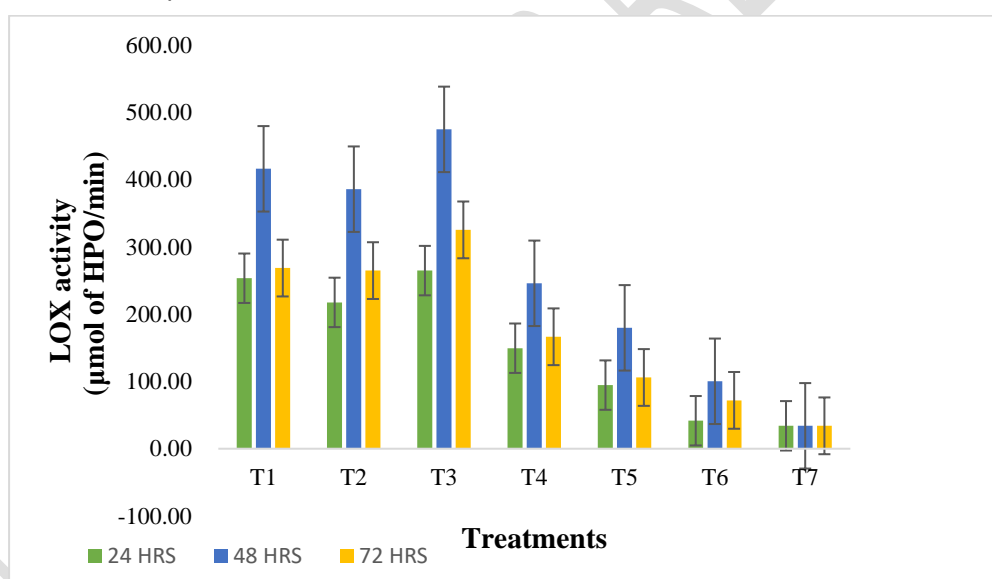
Fig 3. Lipoxygenase enzyme activity in different treatments
