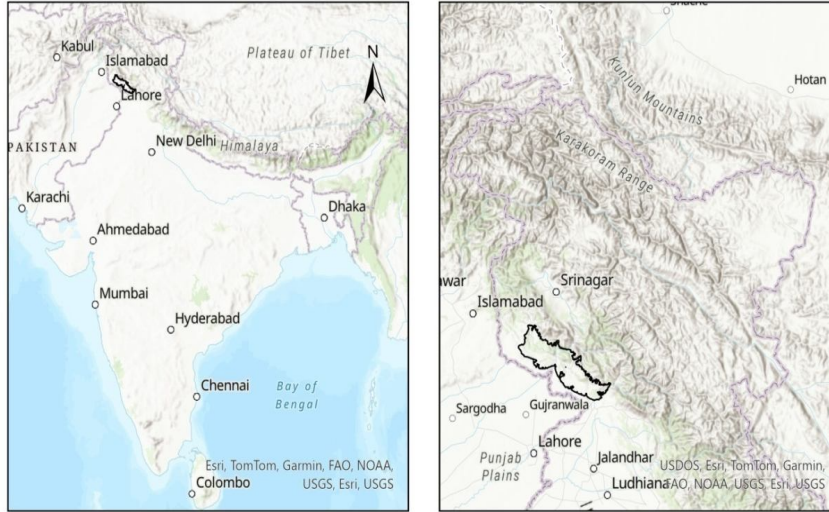
Fig. 1: Location and extent of outer Himalayas
