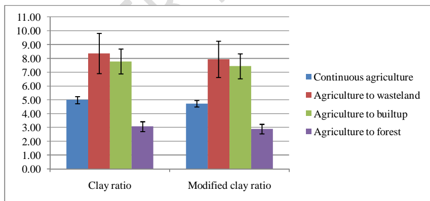
Fig. 3: Clay ratio and Modified clay ratio in continuous agriculture and landuse conversion from agriculture
